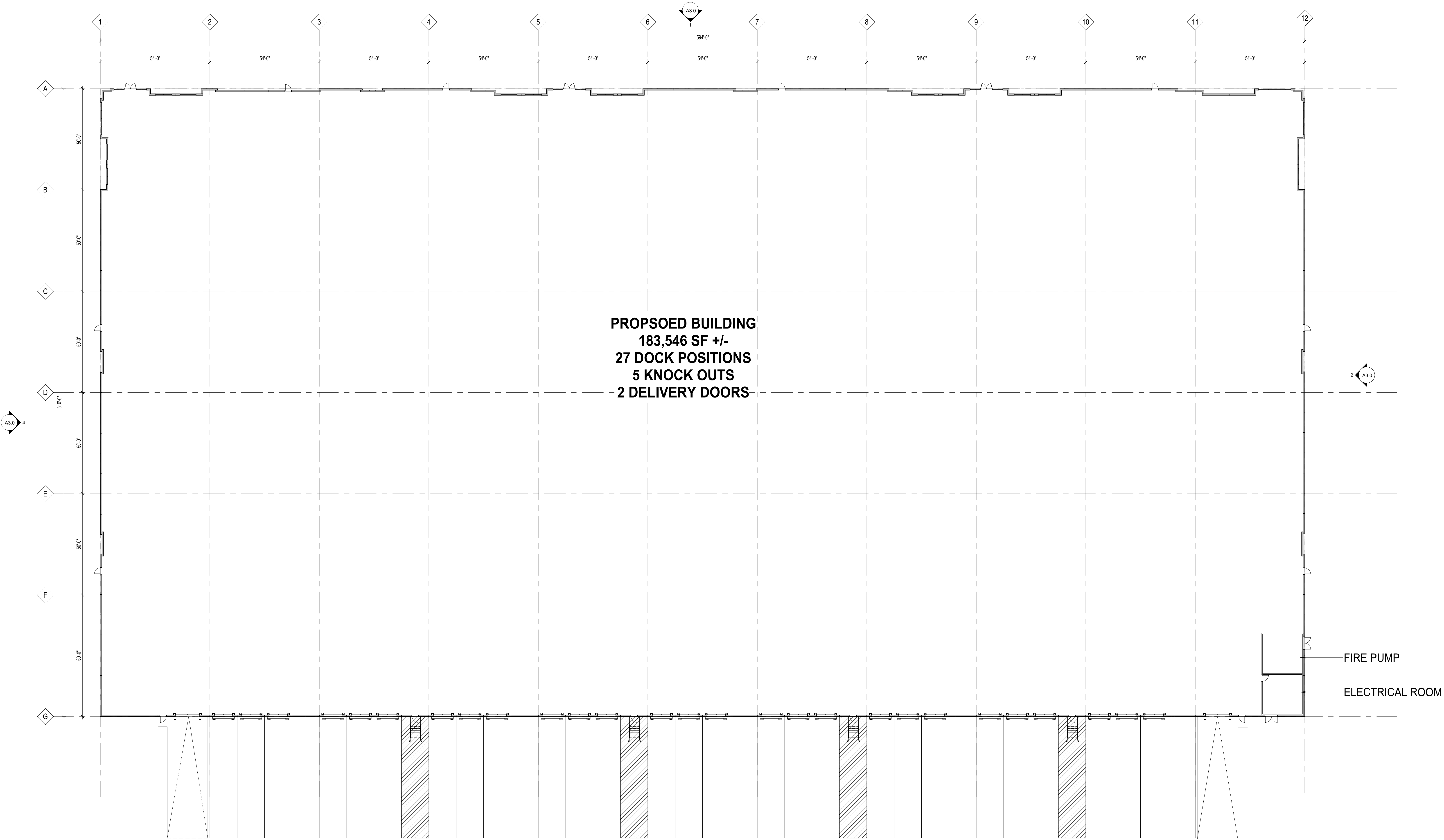
1 A1.0 3/64" = 1'-0"
