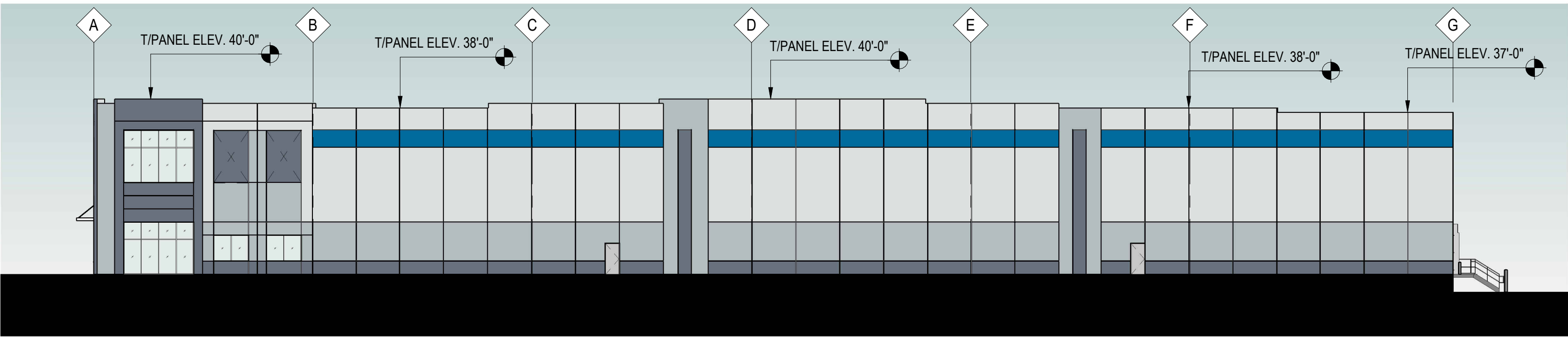
4 NORTH ELEVATION A3.0 3/64" = 1'-0"
