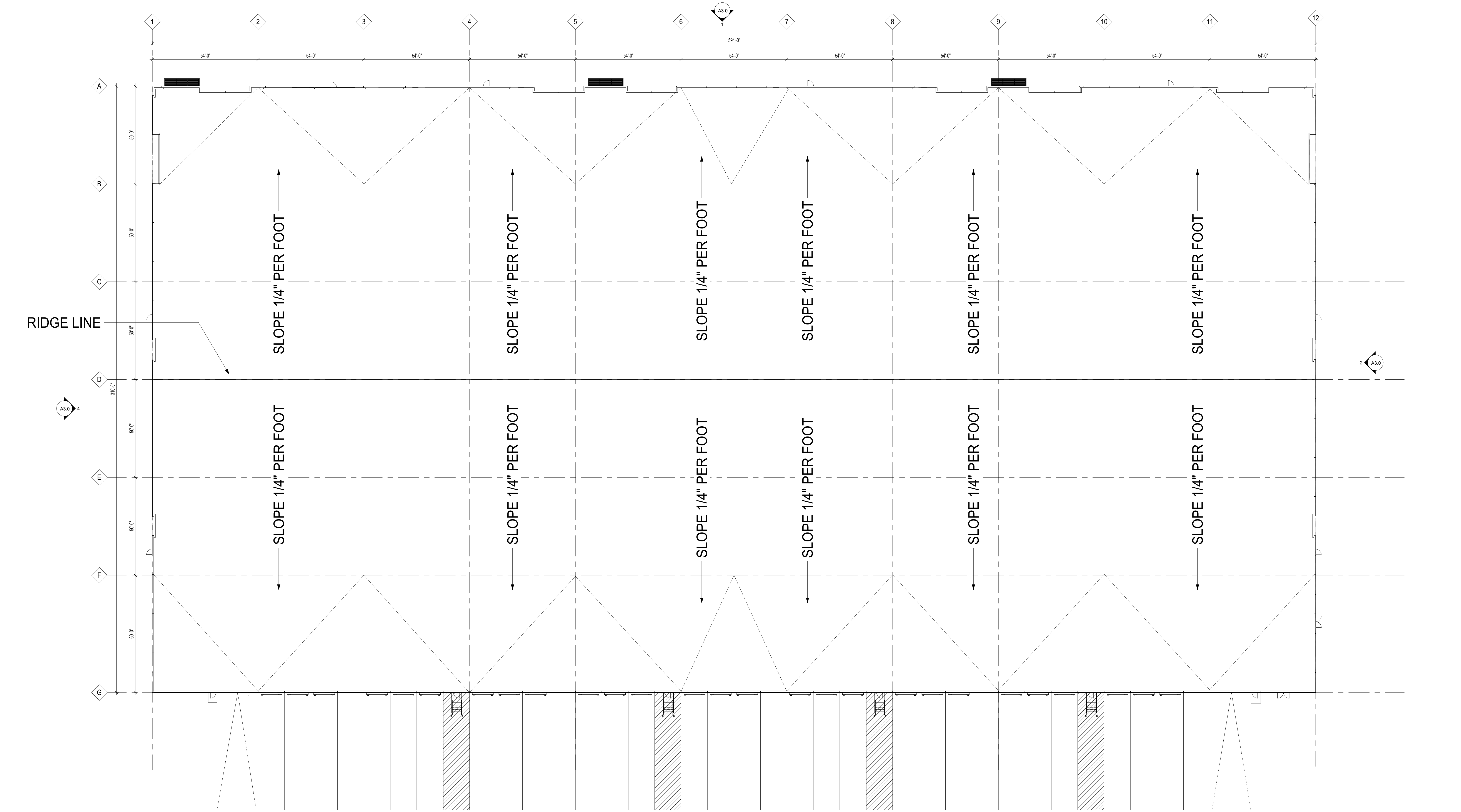
1 PROPOSED ROOF PLAN A2.0 3/64" = 1'-0"
