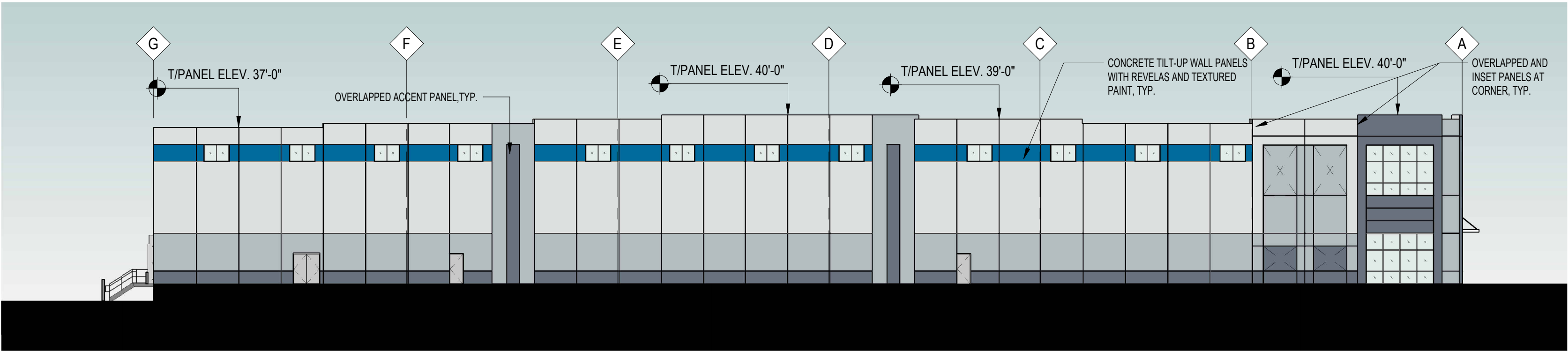
2 SOUTH ELEVATION A3.0 3/64" = 1'-0"
