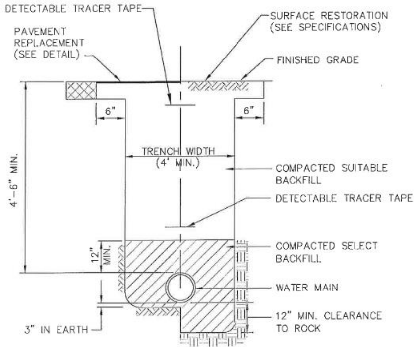
TYPICAL WATER MAIN TRENCH N.T.S.
