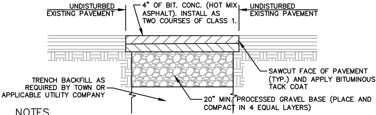
TEMPORARY PAVEMENT DETAIL (DWG. NO. U-1)
