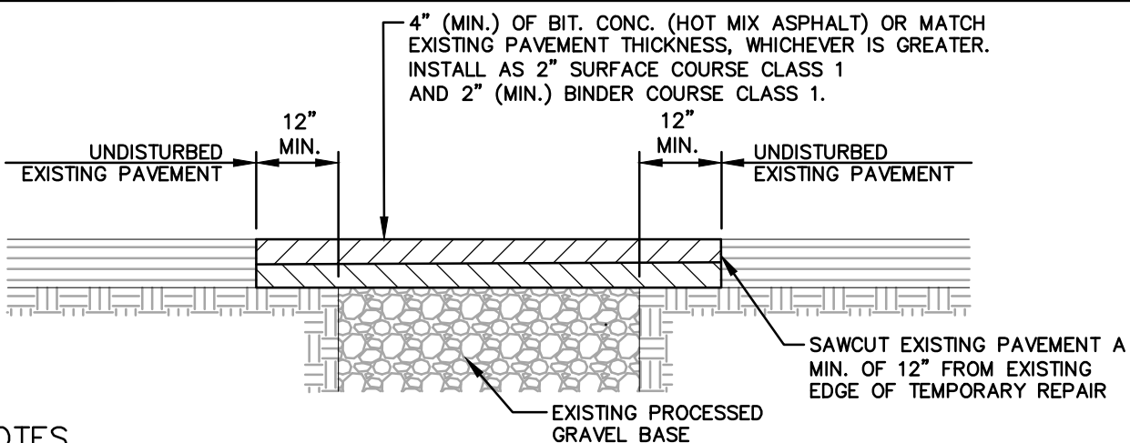
TEMPORARY PAVEMENT DETAIL (DWG. NO. U-1)
